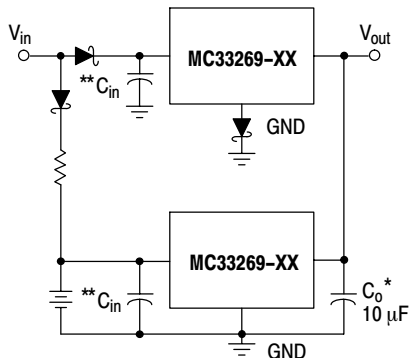
The Schottky diode in series with the ground leg of the upper regulator shifts its output voltage higher by the forward voltage drop of the diode. This will cause the lower device to remain off until the input voltage is removed.
