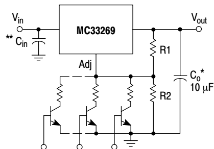
R 2 sets the maximum output voltage. Each transistor reduces the output voltage when turned on.
