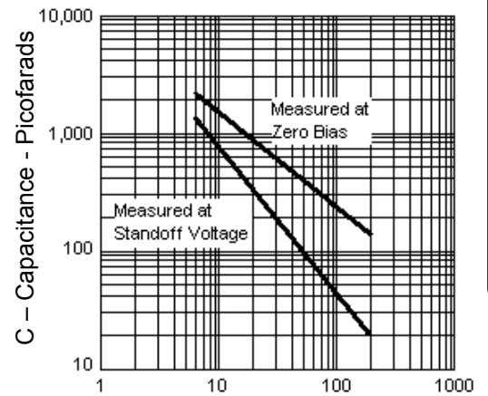
FIGURE 4 Typical Capacitance vs. Breakdown Voltage
