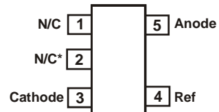
ZTL431_E5 SOT235 (Top View)
