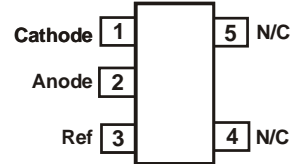
ZTL431_E5 SOT235 (Top View)
