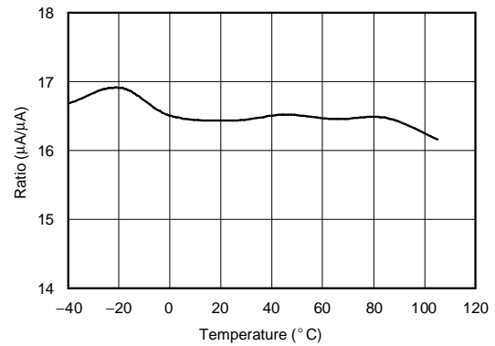
SENSOR BIAS CURRENT SOURCE RATIO vs TEMPERATURE
