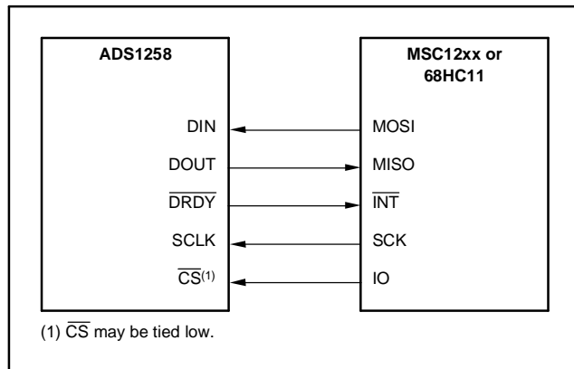
Figure 63. Connection to Microcontrollers with an SPI Interface
