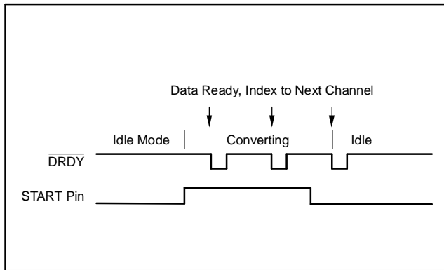
Figure 53. Conversion Control, Auto-Scan Mode
