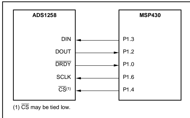
Figure 62. Connection to MSP430 Microcontroller
