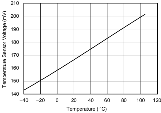
TEMPERATURE SENSOR VOLTAGE vs TEMPERATURE
