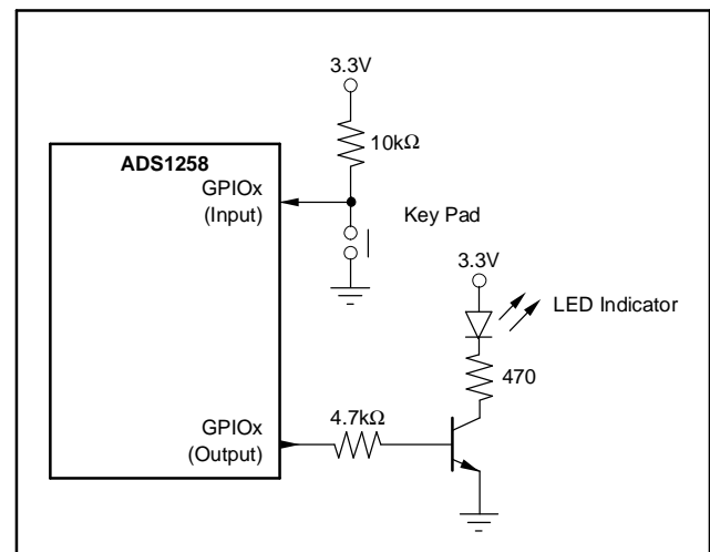
Figure 65. GPIO Connections
