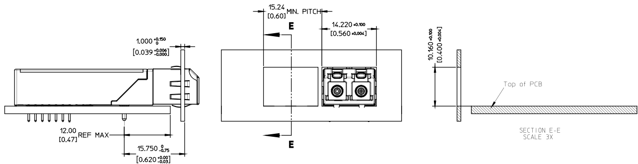
Figure 7. Assembly Drawing
