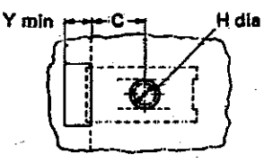
PANEL LAYOUT FOR EDGE OR CENTRE MOUNTING
