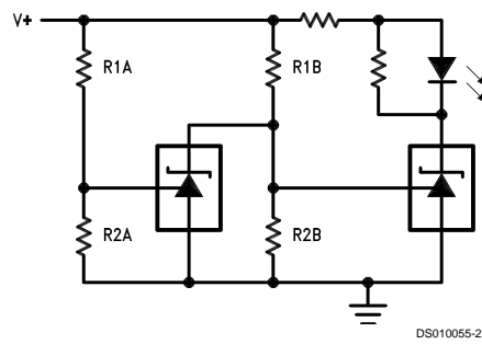
Voltage Monitor
