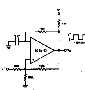
Squarewave Oscillator
