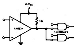
Driving TTL
