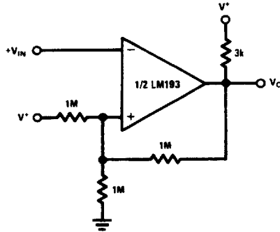
Inverting Comparator with Hysteresis
