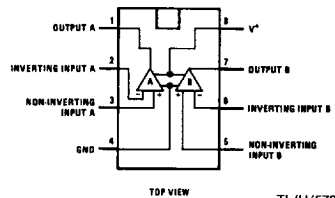
Dual-In-Line Package
