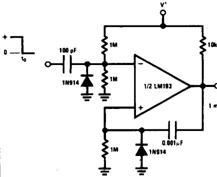
One-Shot Multivibrator
