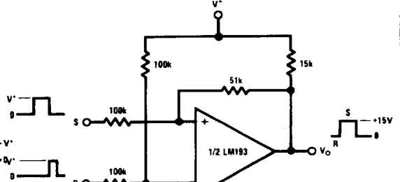
Bi-Stable Multivibrator
