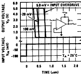
Response Time for Various Input Overdrives—Negative Transition
