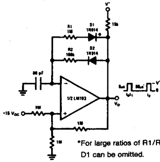
Pulse Generator
