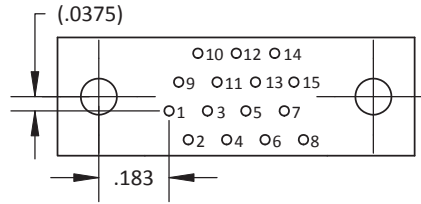
15 CONTACTS
