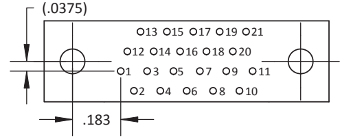
21 CONTACTS
