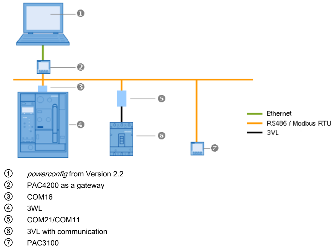
Figure 7-5 LAN/RS485 gateway
