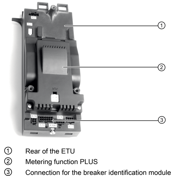
Figure 3-8 Metering function PLUS
