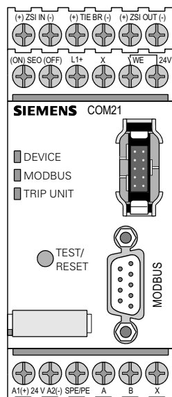
Figure 4-3 MODBUS COM21
