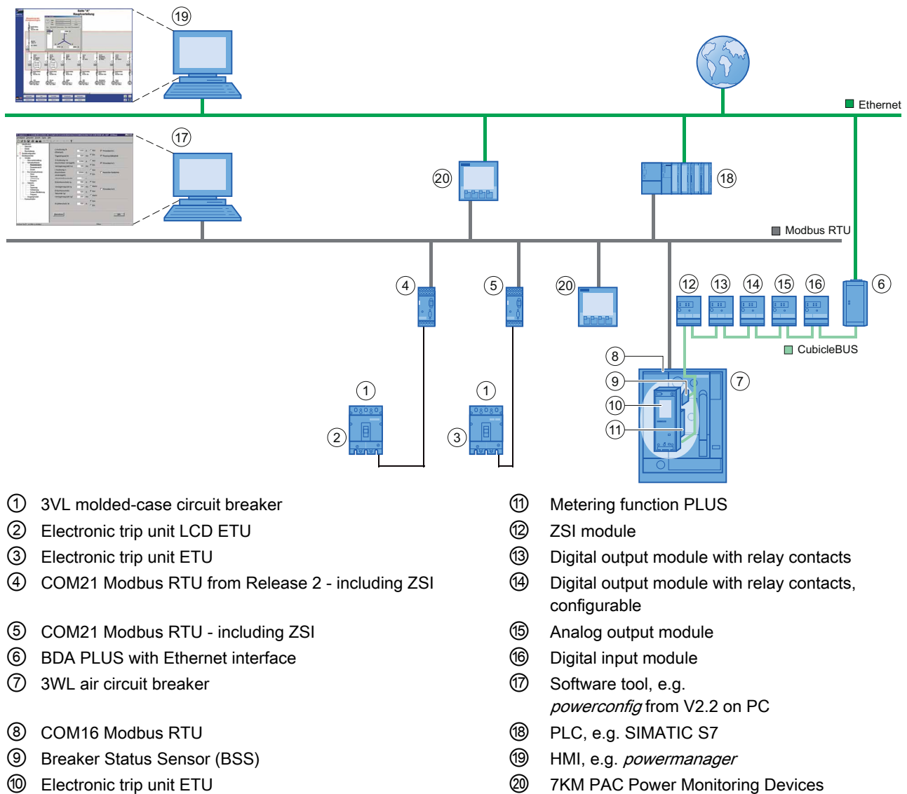
Figure 1-2 System architecture of the SENTRON circuit breakers - Modbus RTU
