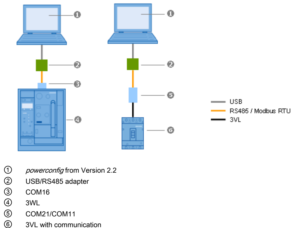
Figure 7-3 USB/RS485 adapter as point-to-point link
