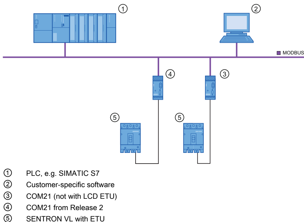
Figure 4-1 System architecture of the SETRON VL
