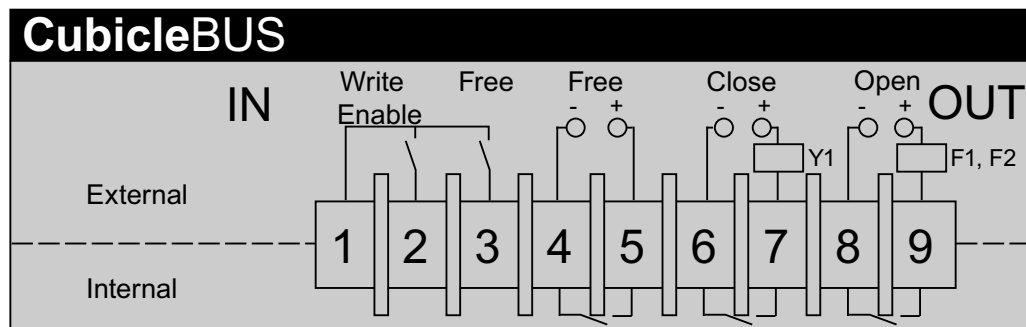
Figure 3-2 COM16 pin assignment
