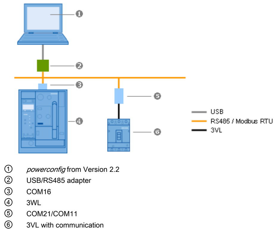
Figure 7-4 USB/RS485 adapter
