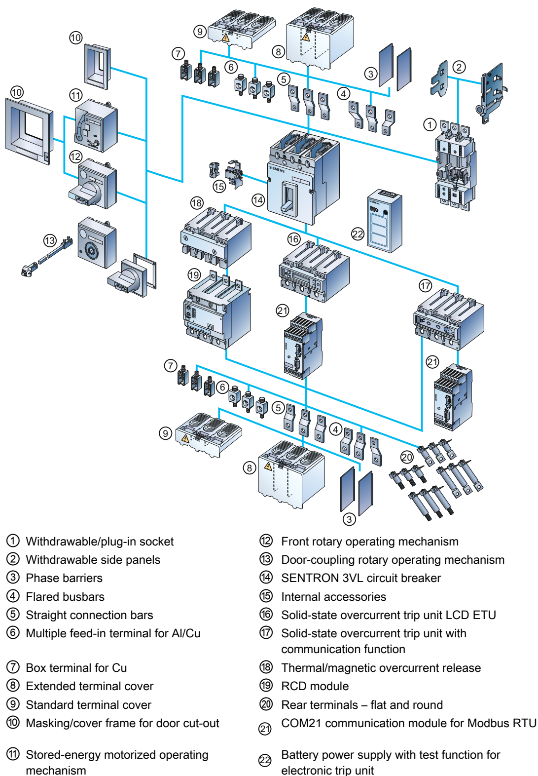
Figure 4-2 SENTRON VL, accessories
