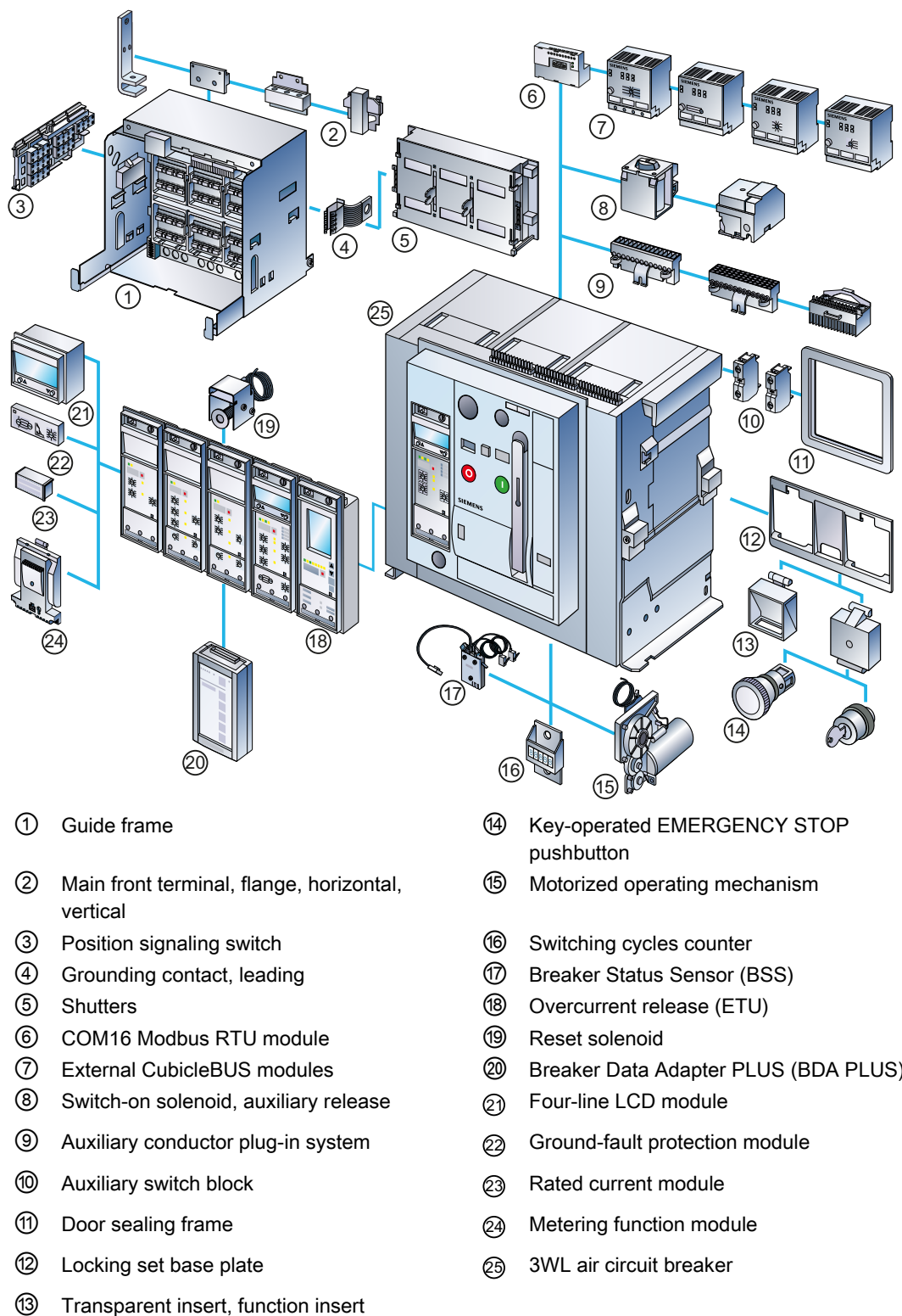
Figure 3-1 SETRON WL, accessories
