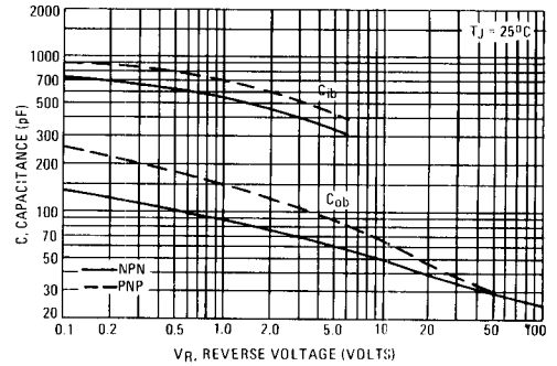
FIGURE 5 — CAPACITANCE
