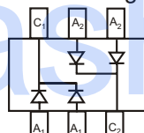
BAT54CDW* Marking: KL7
