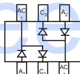
BAT54SDW* Marking: KL8
