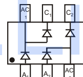
BAT54BRW Marking: KLB
