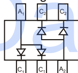
BAT54ADW* Marking: KL6
