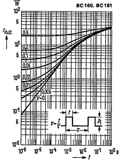
Permissible pulse load i_{thJC} = f(t); v = \text{parameter}
