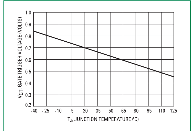
Figure 7. Typical Gate Trigger Voltage vs. Junction Temperature
