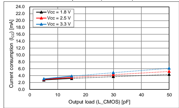
T_{use} = +25\text{ }^{\circ}\text{C} , Output load ( L_{CMOS} ) Characteristics
