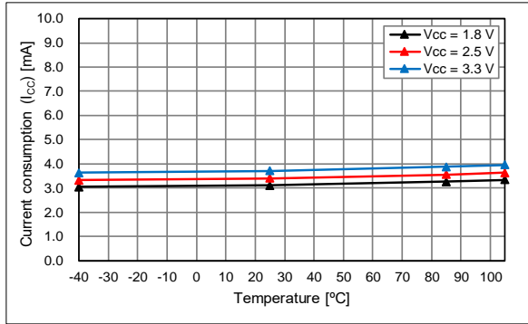
L_{CMOS} = 5\text{ pF} , Temperature Characteristic
