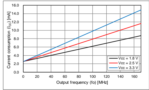
L_{CMOS} = 15\text{ pF} , T_{use} = +25\text{ }^{\circ}\text{C} , Freq. Dependency
