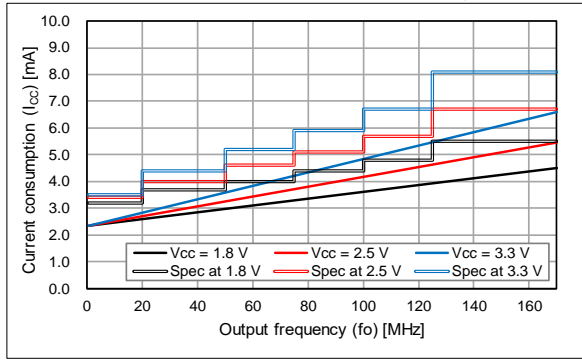
No load, T_{use} = +25\text{ }^{\circ}\text{C} , Freq. Dependency
