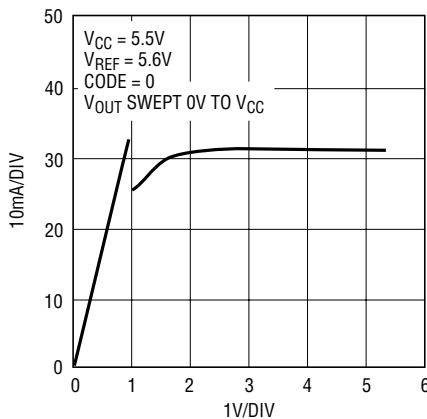
Short-Circuit Output Current vs VOUT (Sinking)
