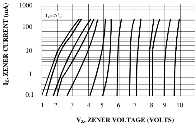
Figure 8. Zener Voltage versus Zener Current V_Z=3.3 thru 10 Volts
