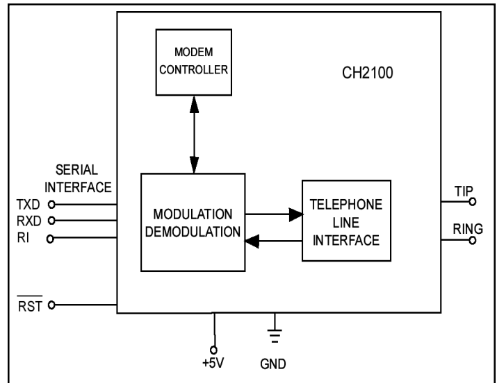
Figure 1. Functional Block Diagram of CH2100.
