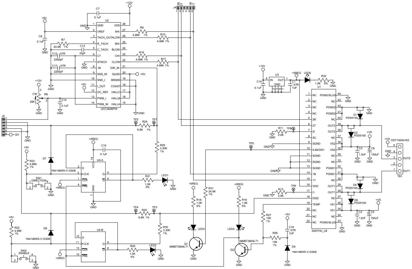
Figure 2 – Schematic
