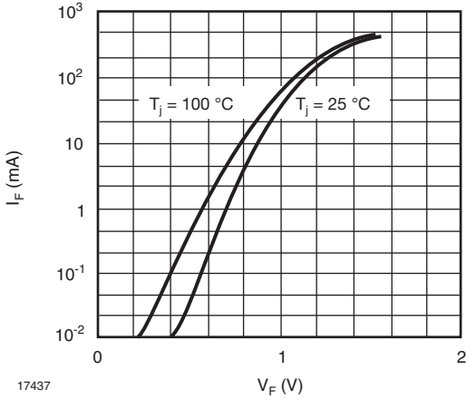
Fig. 1 - Forward characteristics
