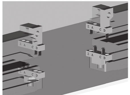
CCKP32-CD mates with CCKJ32-CD
