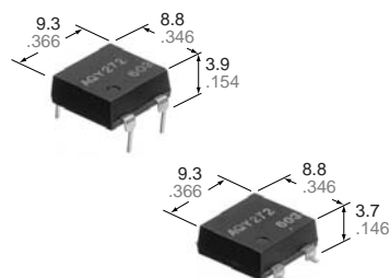
mm inch
