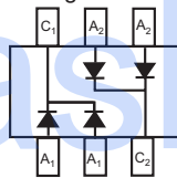
BAT54CDW* Marking: KL7
