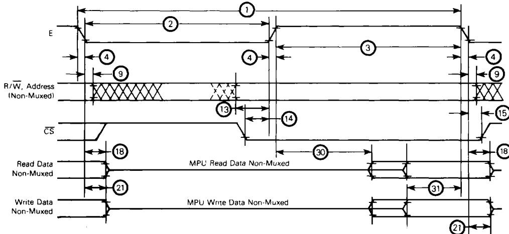
FIGURE 1 — BUS TIMING
