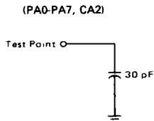
FIGURE 4 — CMOS EQUIVALENT TEST LOAD
