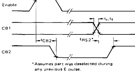
FIGURE 12 — CB2 DELAY TIME (Write Mode; CRB-5=1, CRB-3=CRB-4=0)
