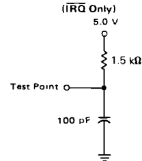
FIGURE 5 — NMOS EQUIVALENT TEST LOAD
