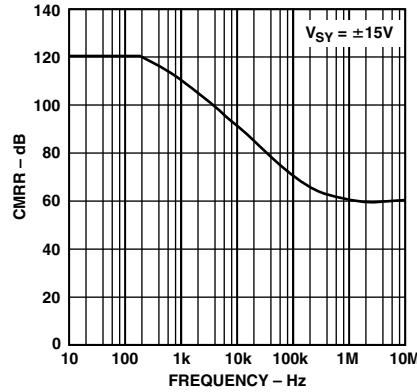
TPC 14. CMRR vs. Frequency
