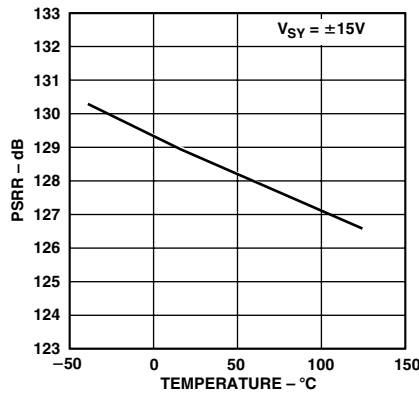
TPC 23. PSRR vs. Temperature
