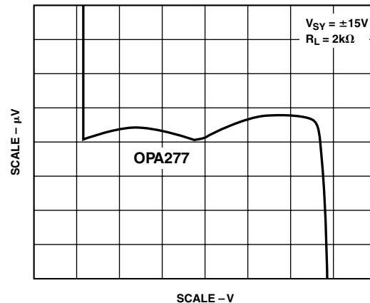
Figure 2. Gain Linearity
