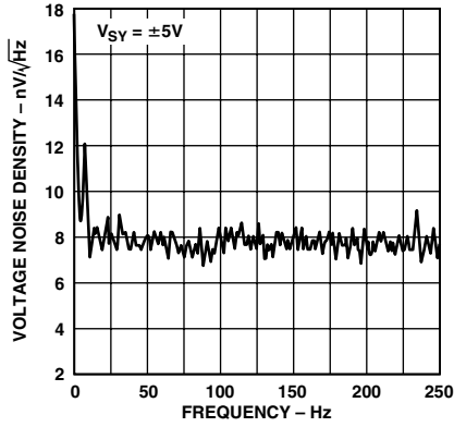
TPC 38. Voltage Noise Density
