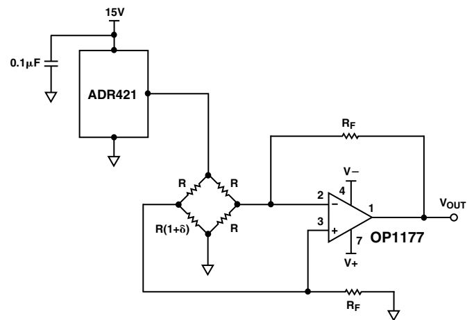
Figure 16. Single Bridge Amplifier
