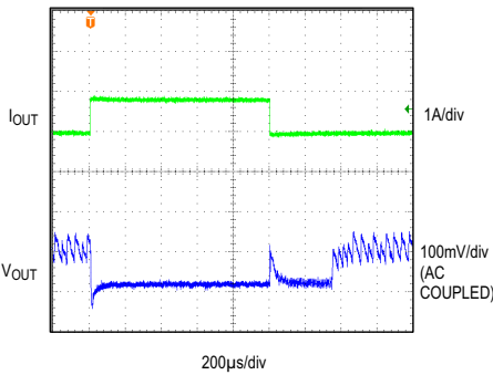
LOAD CURRENT TRANSIENT RESPONSE V_{IN} = 24V, V_{OUT} = 5V, I_{OUT} = 0.05A - 0.85A, MODE = OPEN
