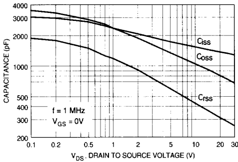
Figure 9. Capacitance Characteristics.
