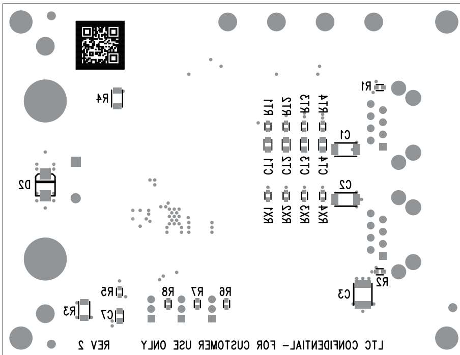
Bottom Silkscreen
