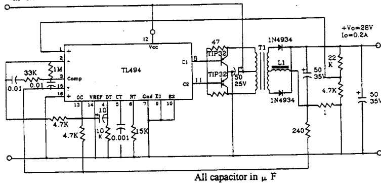
FIGURE 21-PULSE-WIDTH MODULATED PUSH-PULL CONVERTER +Vin=8.0 to 20
