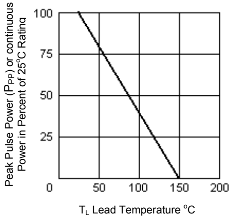
FIGURE 3 - Derating Curve
