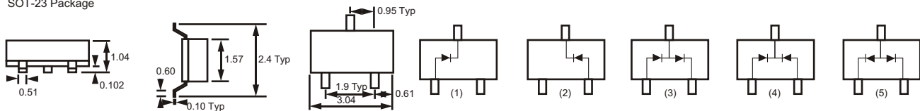
SOT-23 Package
