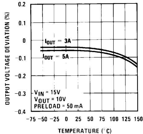
Figure 4. Load Regulation
