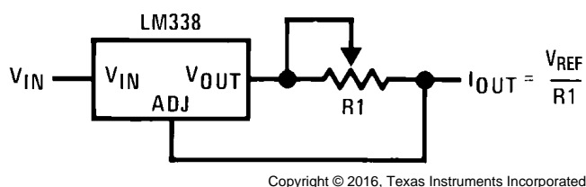
Figure 34. 12-V Battery Charger
