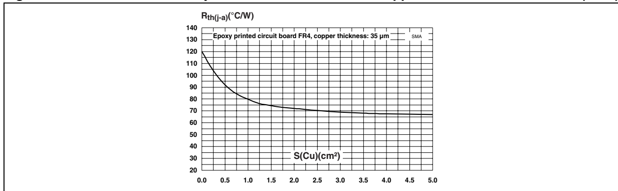
Figure 13. Thermal resistance junction to ambient versus copper surface under each lead (SMA)
