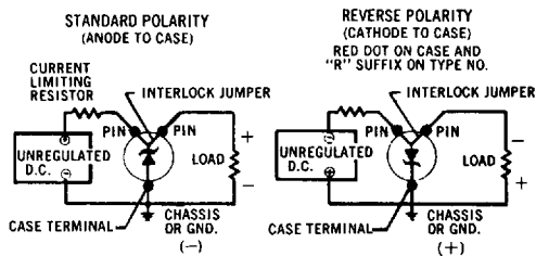
Typical circuit connections for anode-to-case and cathode-to-case polarities (standard and reverse polarities, respectively).
