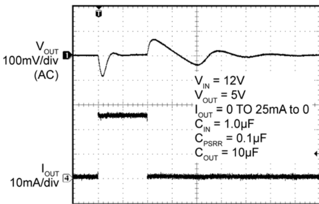
Time (100μs/div)
