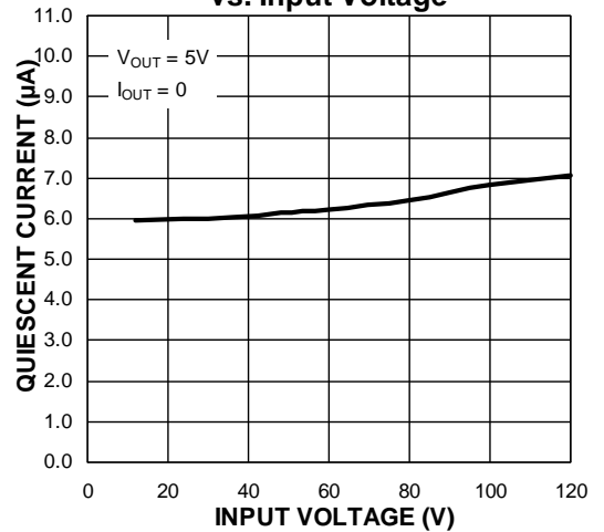
Quiescent Supply Current vs. Input Voltage
