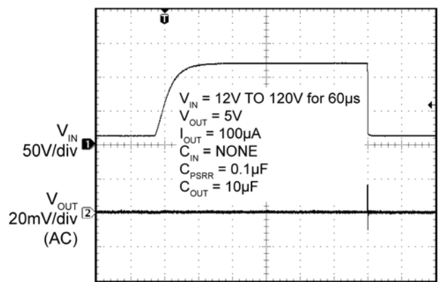
Time (10μs/div)
