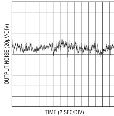
LT1460S3-10V Output Noise 0.1Hz to 10Hz
