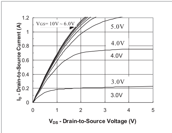
FIG.1- Output Characteristic
