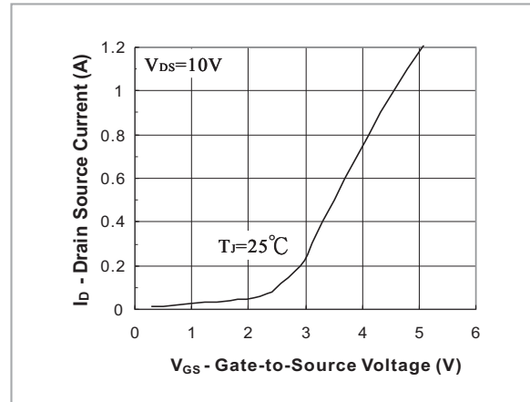
FIG.2- Transfer Characteristic
