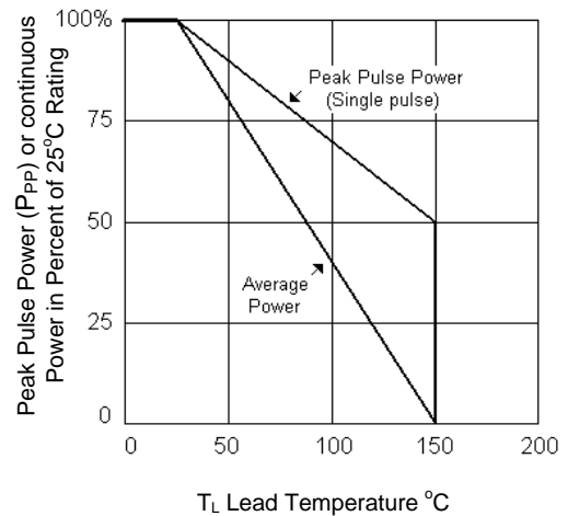
FIGURE 4 Derating
