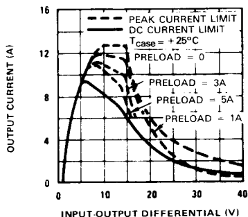
CURRENT LIMIT
