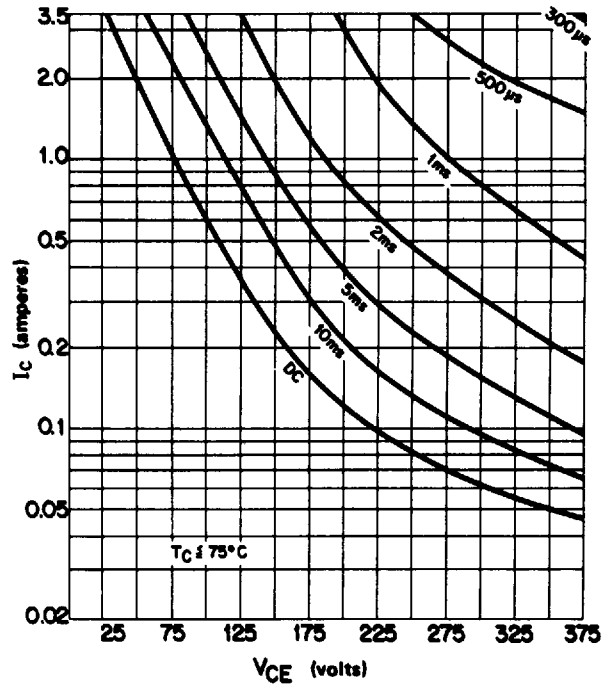
SAFE OPERATING CURVES
