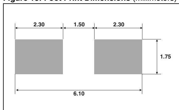
Figure 13: Foot Print Dimensions (millimeters)
