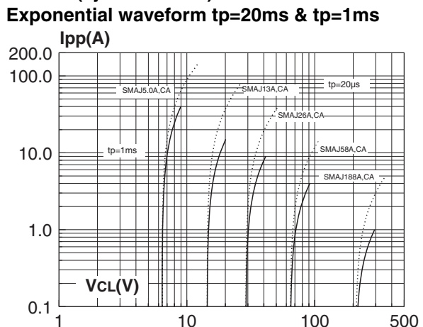
Figure 4: Clamping voltage versus peak pulse current (Tj initial=25°C)
