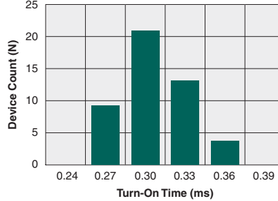
Typical Turn-On Time (N=50, I F =10mA, I L =1A DC )
