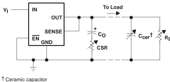
† Ceramic capacitor Figure 6. Test Circuit for Typical Regions of Stability (Refer to Figures 29 through 32)
