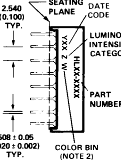
SIDE VIEW E, F, G, H
