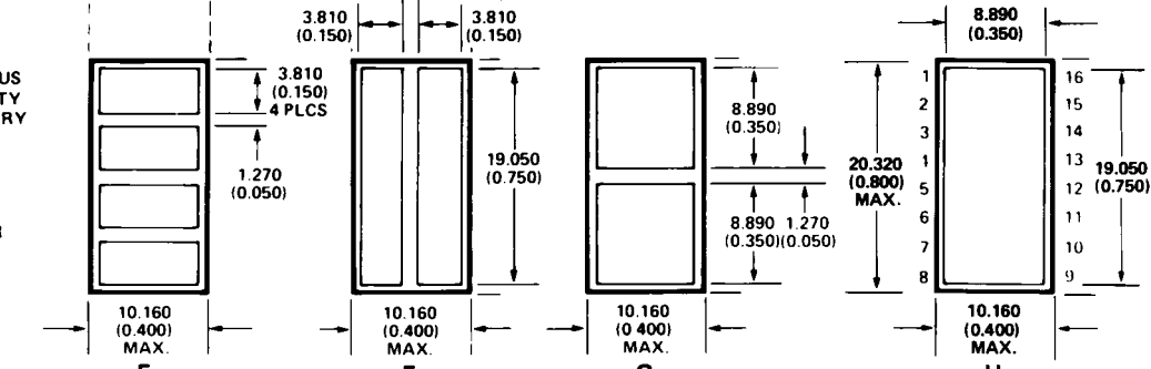
END VIEW C, D, E, F, G, H, I
