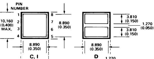
SIDE VIEW C, D, I
