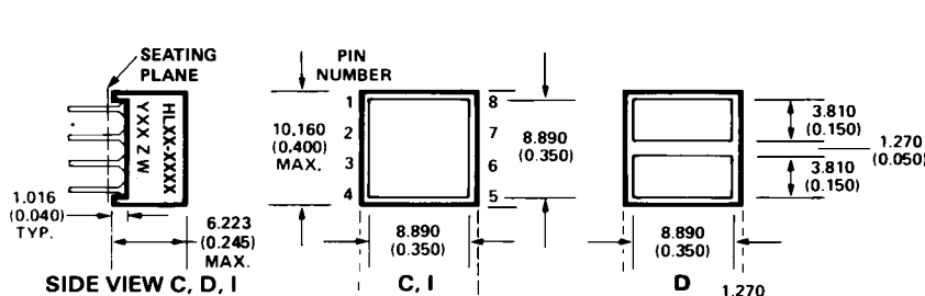
SIDE VIEW C, D, I
