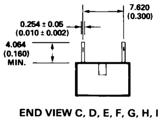
END VIEW C, D, E, F, G, H, I
