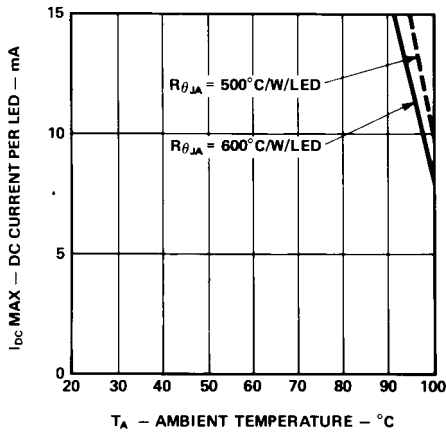
Figure 2. Maximum Allowed DC Current per LED vs. Ambient Temperature, T J MAX = 110 °C.
