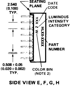
SIDE VIEW E, F, G, H
