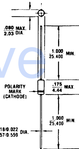
FIGURE 1 All dimensions in \frac{\text{INCH}}{\text{m.m.}}
