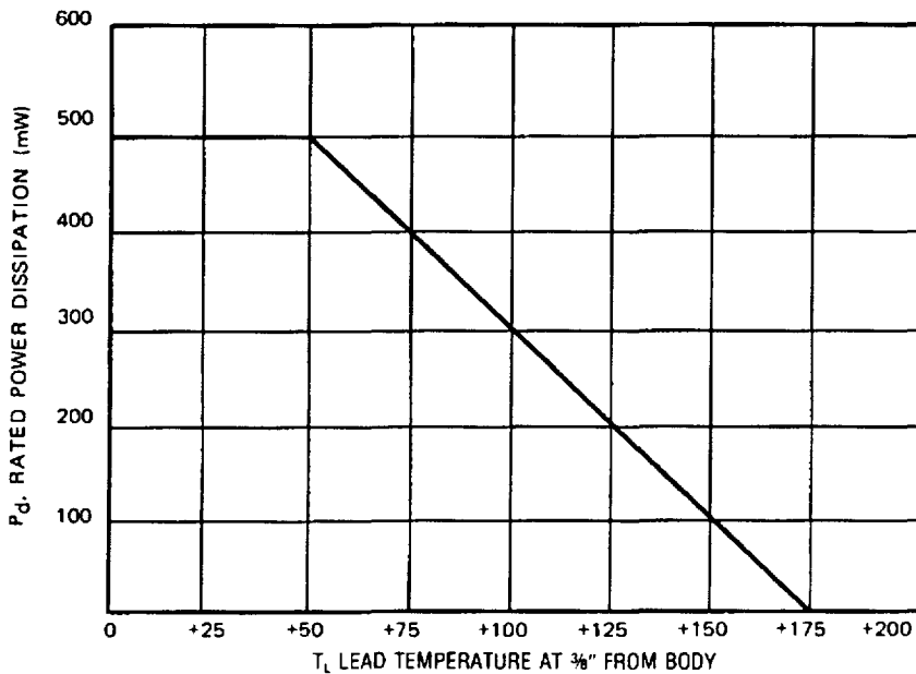
FIGURE 2 POWER DERATING CURVE
