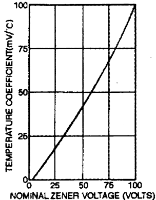
FIGURE 4 TEMP. COEFF. vs. ZENER VOLTAGE
