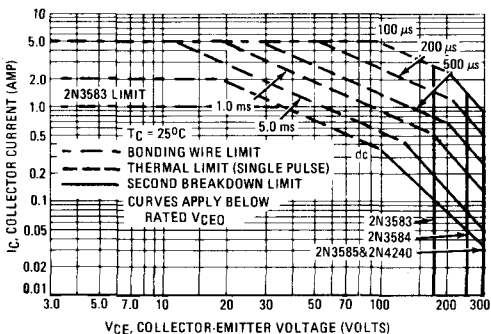
FIGURE 7 — 2N3583 thru 2N3585, 2N4240
