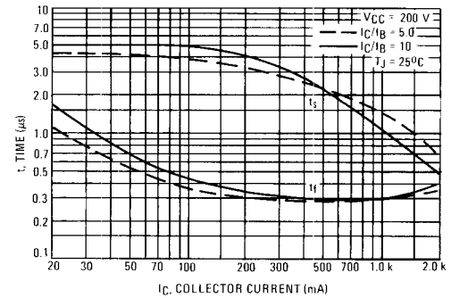
FIGURE 3 — TURN-OFF TIME
