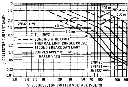
FIGURE 8 — 2N6420 thru 2N6422
