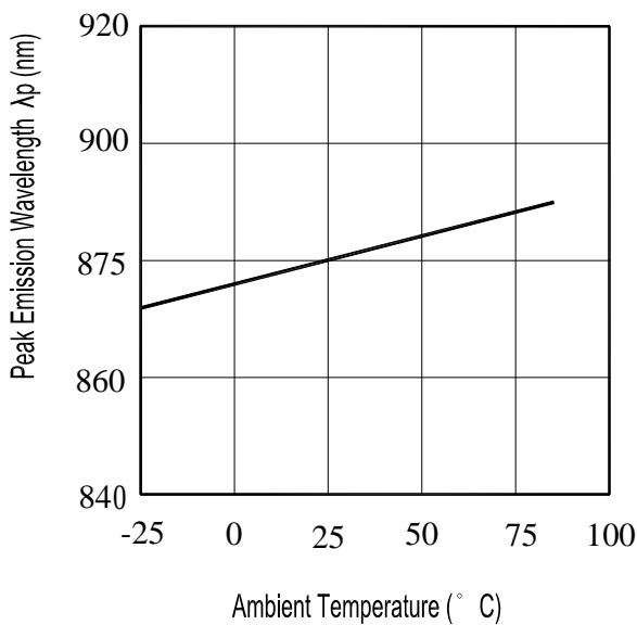
Fig.3 Peak Emission Wavelength λp vs. Ambient Temperature
