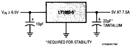
5V, 7.5A Regulator
